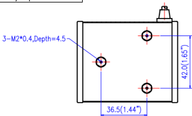
Figure 1: Screw Position
